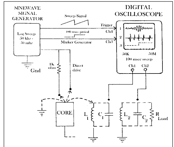
Figure 7. Swept signal analysis setup.
