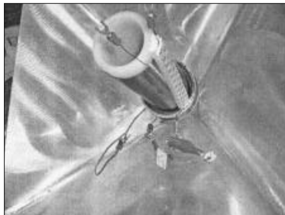
Figure 2. Placement of coils inside the pyramidal charge collector with resonance capacitor.
