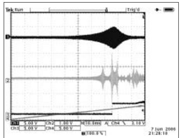
Figure 8. Swept signal analysis of coil resonances and energy transfer.
