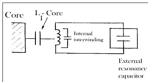
Figure 6. The lumped-element resonant circuit model.
